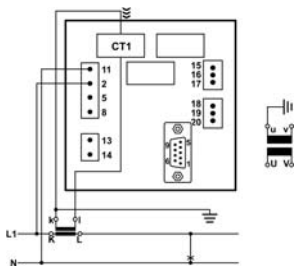
1b – single wire, uniform load
