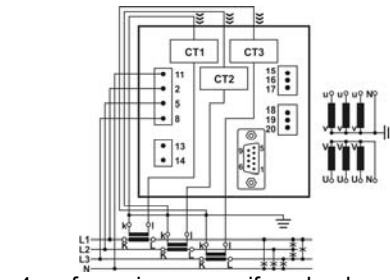
4u – four-wire, non-uniform load
