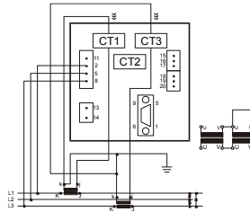
3u – three-wire, non-uniform load
