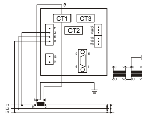
3b – three-wire, uniform load
