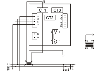
4b – four-wire, uniform load
