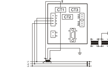
3b – three-wire, uniform load
