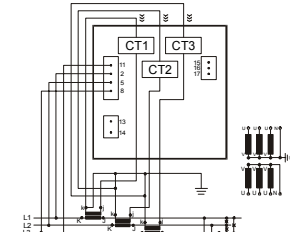
4u – four-wire, non-uniform load
