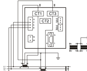
3u – three-wire, non-uniform load
